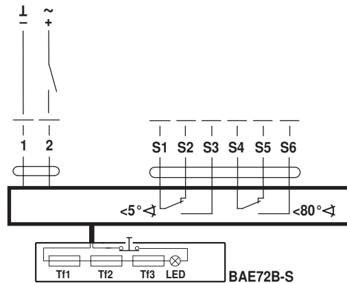
Wiring diagram
