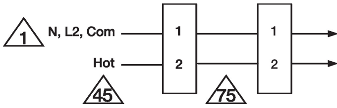
Parallel Actuator Wiring
