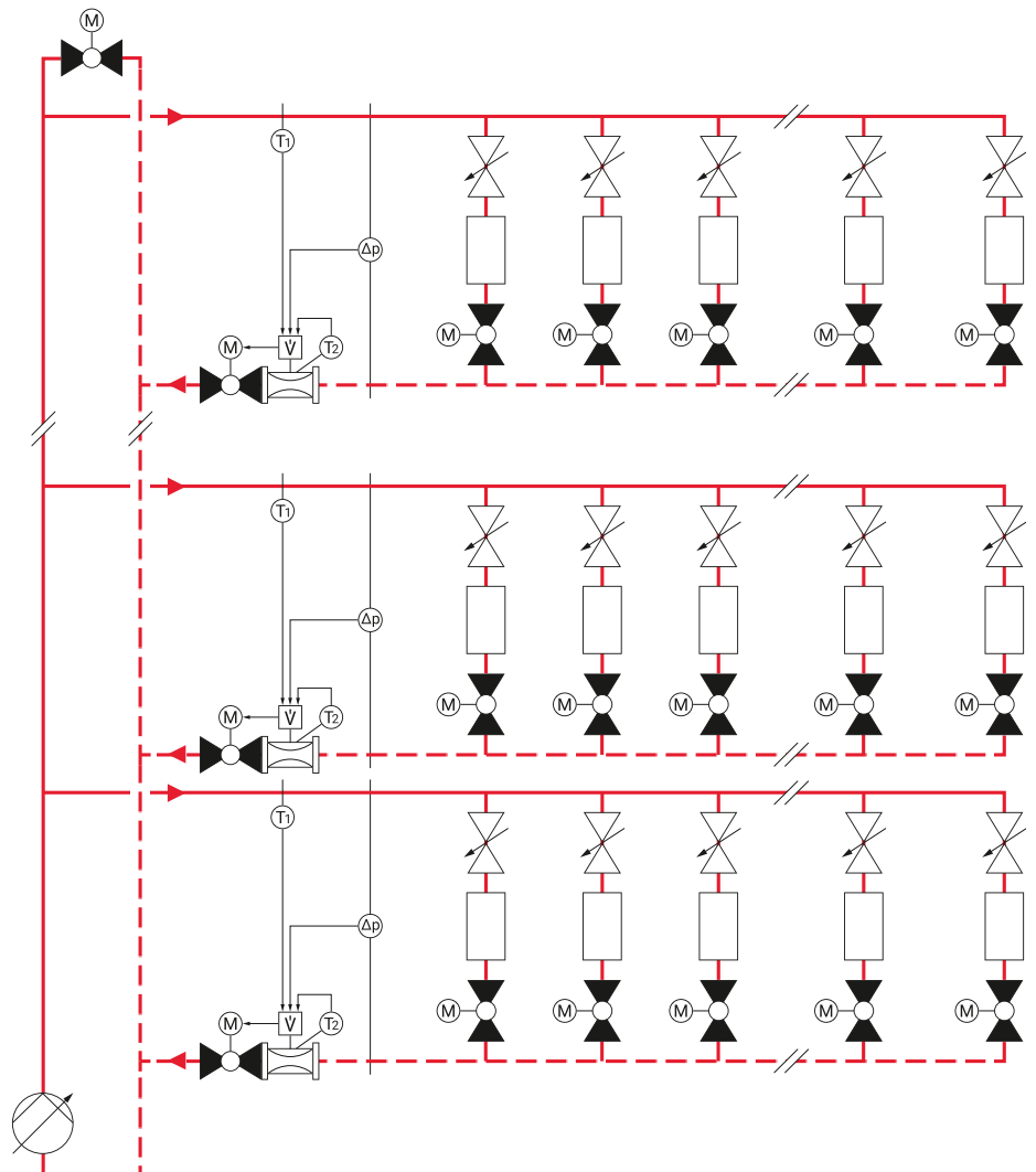
Dynamic balancing of the system segment (building floor) and static balancing of the coils
