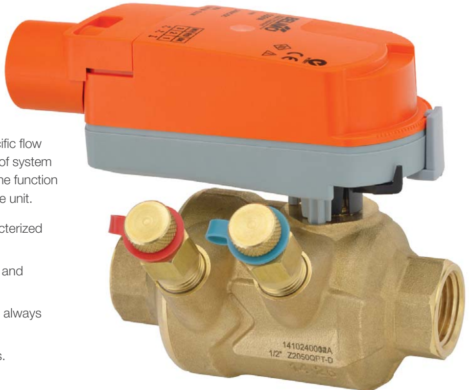
Actual Size PIQCV with Non-Spring Return Actuator
