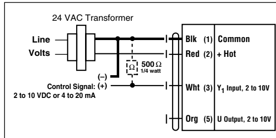
VDC/4-20 mA
