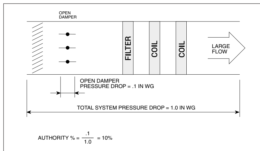
Figure 5B. Damper Pressure Drop
