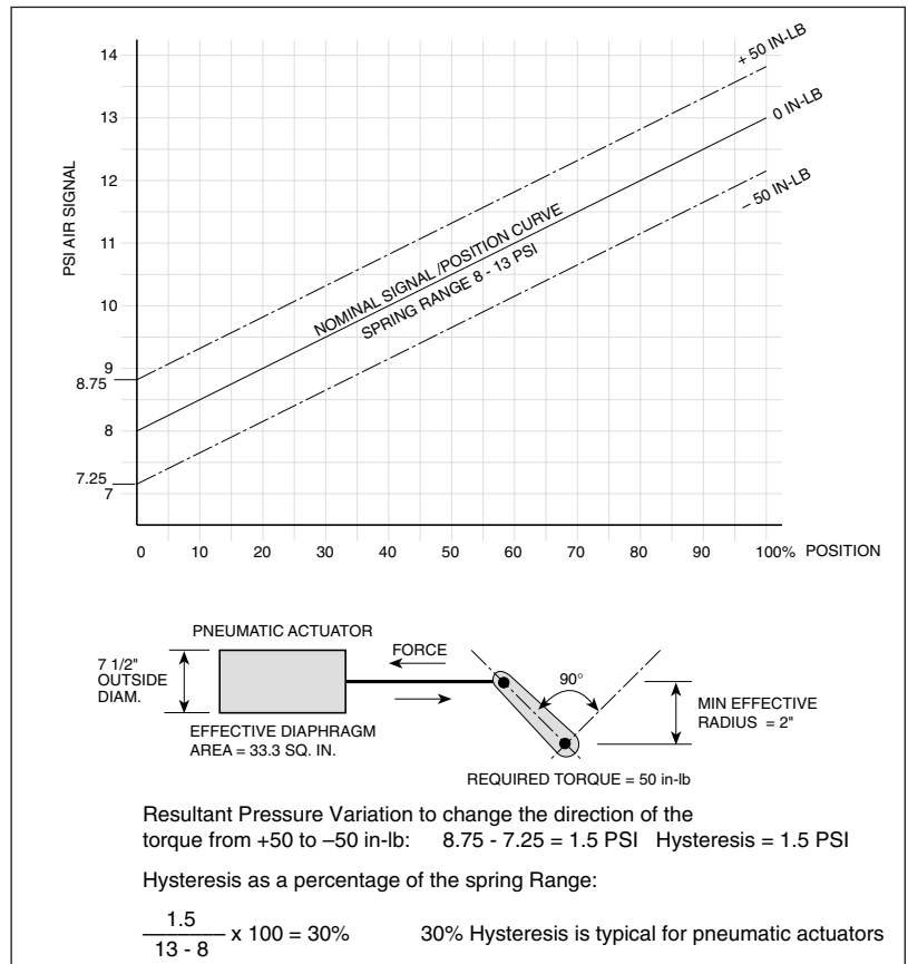
Figure 15. Typical Pneumatic Spring Range Shift and Hysteresis
