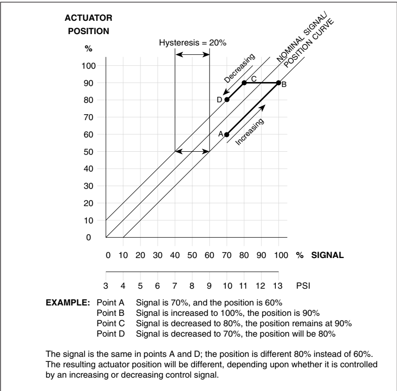
Figure 13. Hysteresis
