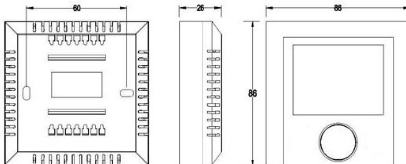
Figure 2: Dimensions in mm
