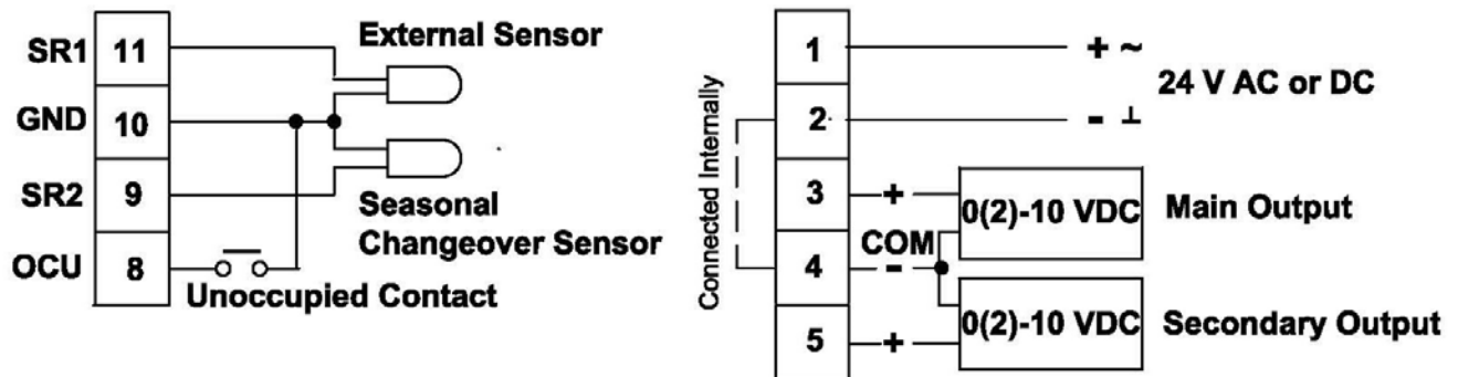
Figure 8: Wiring Diagrams
