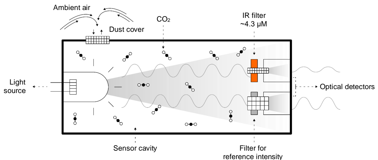
Figure 1: Visualization of the NDIR dual detector approach
