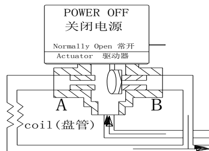
Fig. 6: 3-way valve in Diverting Configuration, Normally Open to coil 图 6: 三通阀分流布置(常开)管道安装
