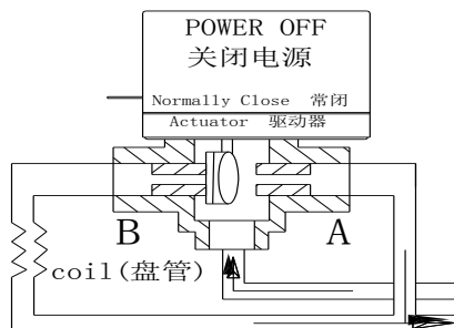
Fig. 5: 3-way valve in Diverting Configuration, Normally Closed to coil 图 5: 三通阀分流布置(常闭)管道安装
