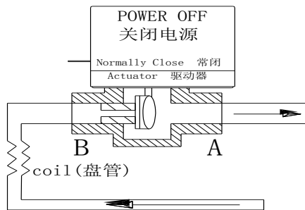
Fig. 1: 2-way Normally Closed to the Coil 图 1: 二通阀(常闭)管道安装
