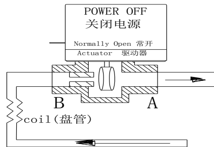
Fig. 2: 2-way Normally Open to the Coil 图 2: 二通阀(常开)管道安装
