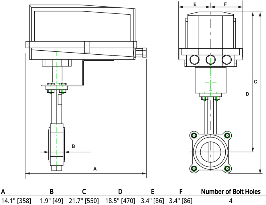
Valve with DR N4/GR N4/GK N4 Actuator
