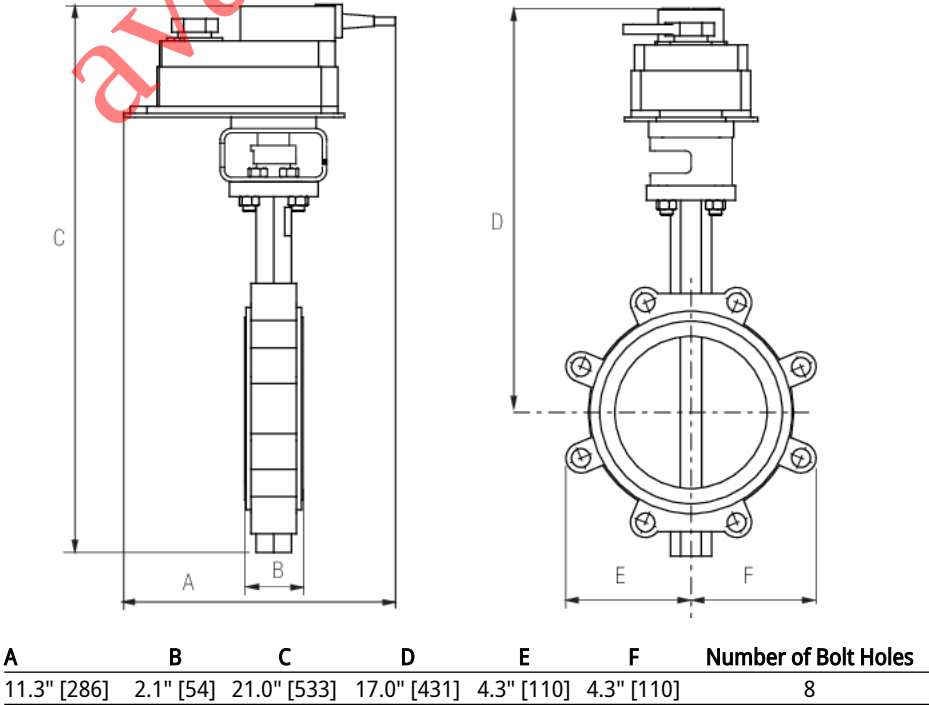
Valve with DR/DK Actuator
