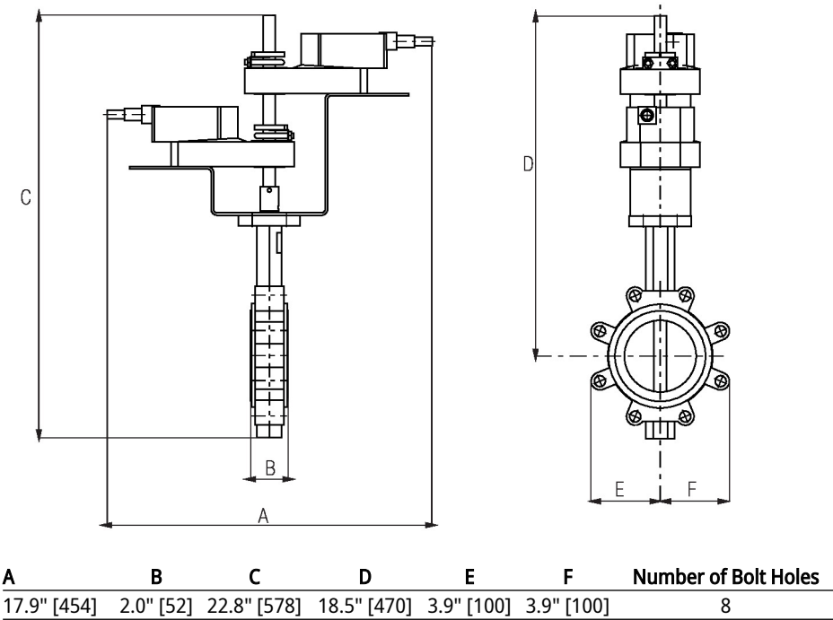
Valve with 2*GK/2*GM Actuator
