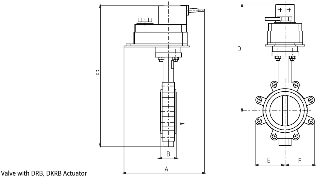
Valve with DRB, DKRB Actuator
