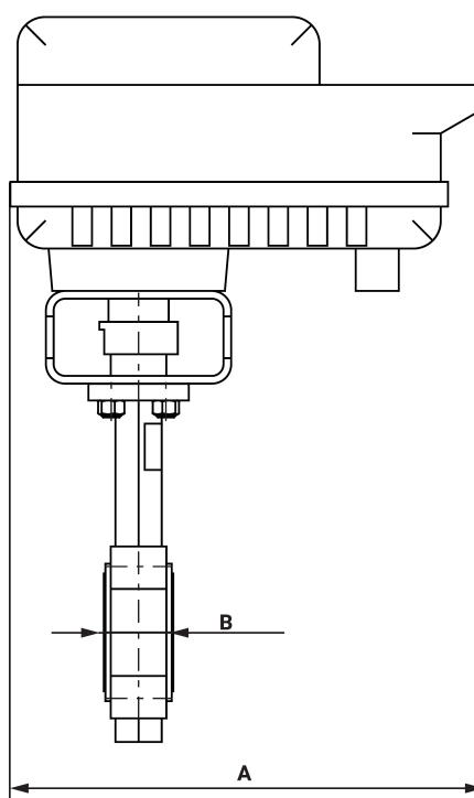
Valve with PK Actuator
