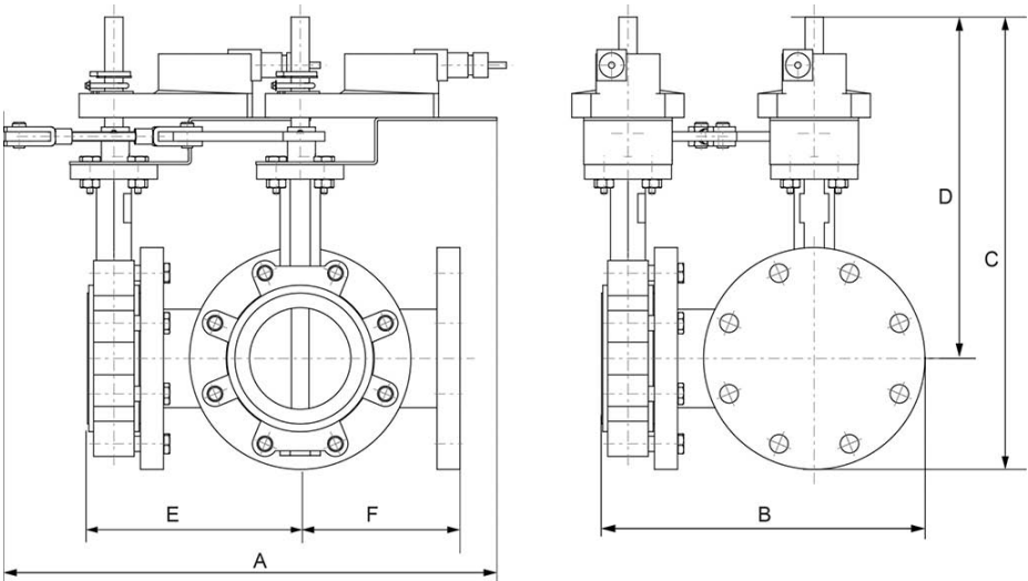
Valve with 2*GMX24-MFT-X1 Actuator
