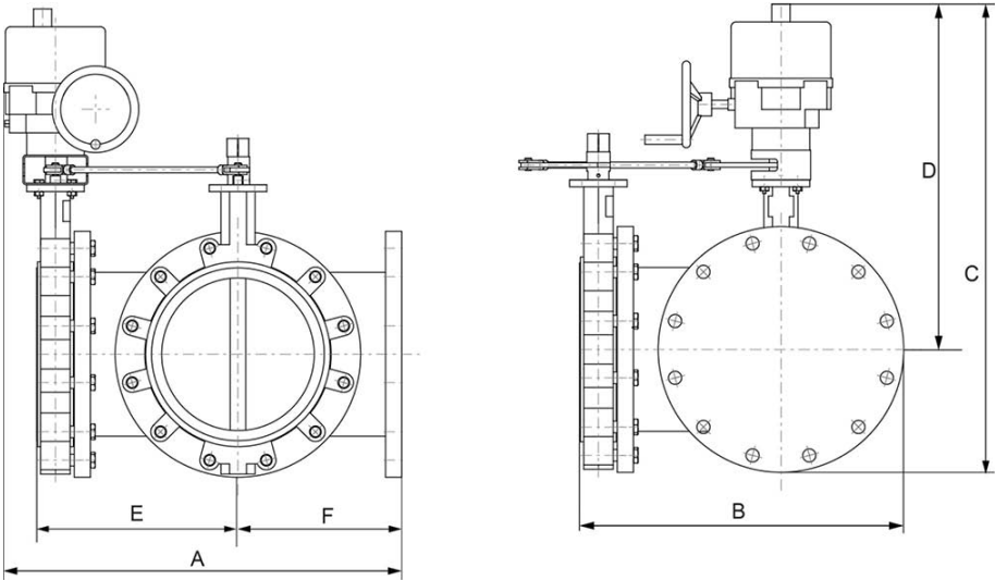
Valve with SY6 Actuator
