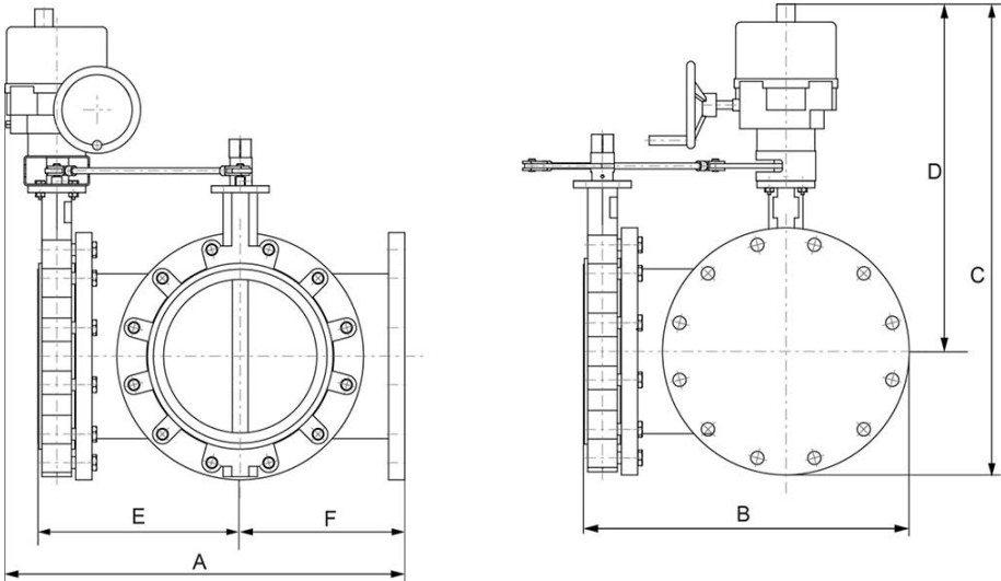
Valve with SY6 Actuator
