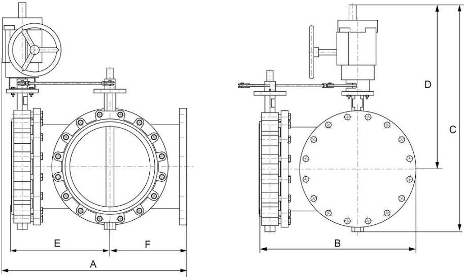
Valve with SY8 Actuator
