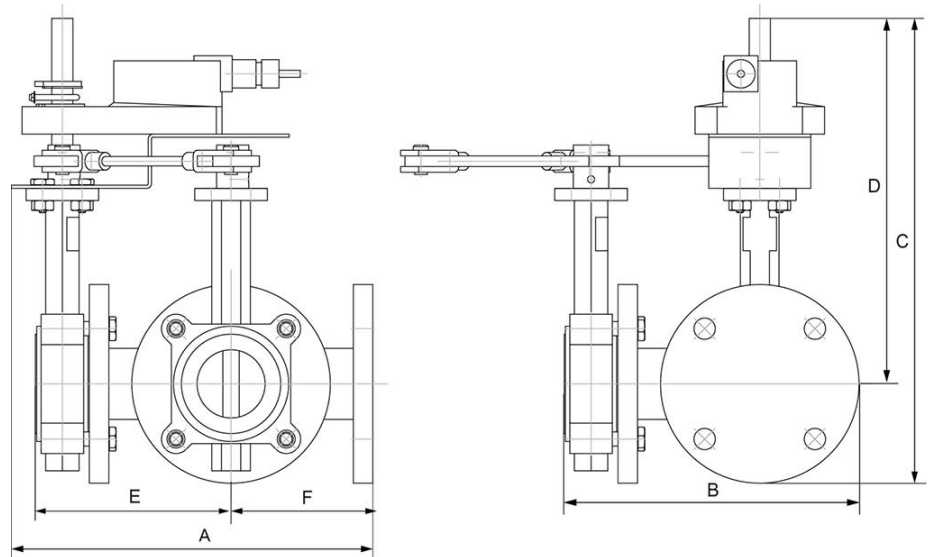
Valve with AM/GM Actuator
