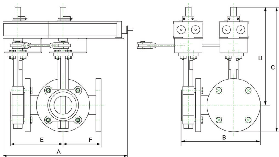
Valve with 2*AFX Actuator
