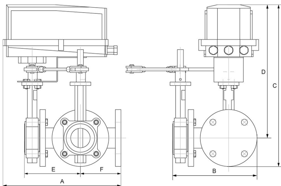
Valve with GM..N4 Actuator
