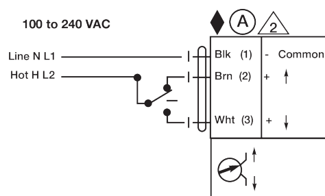
Floating Point
