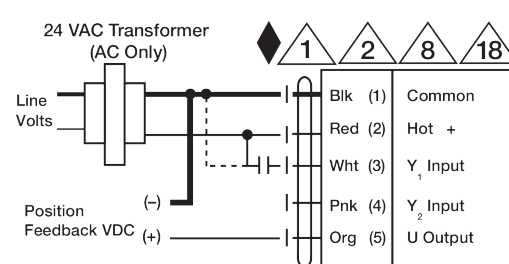
Control PWM
