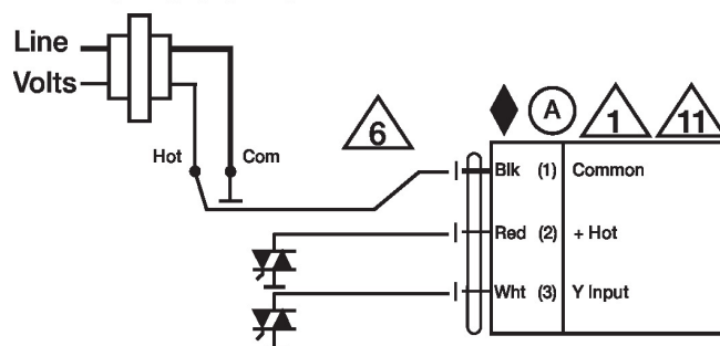
24 VAC Transformer
