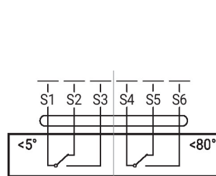
Auxiliary switch
