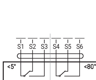
Auxiliary switch
