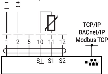
Connection of passive sensors
