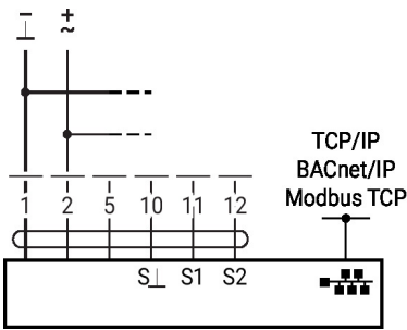
Connection of active sensors
