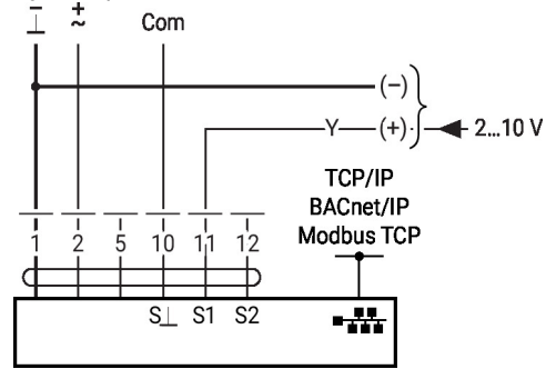
Switching contact connection
