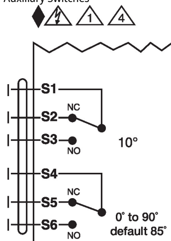
Auxiliary Switches
