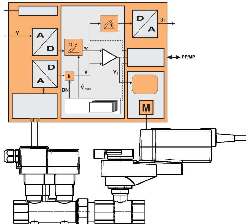
Block diagram
