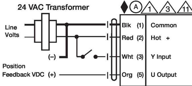
VDC/mA Commande
